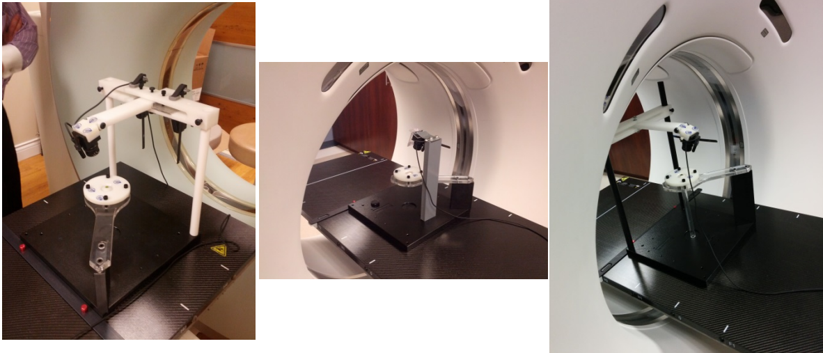
Figure 21: 1st version Setup for CT scan (Left), Improved version with a single upright beam (Middle), and the Latest Version with Tight Screws (Right).
